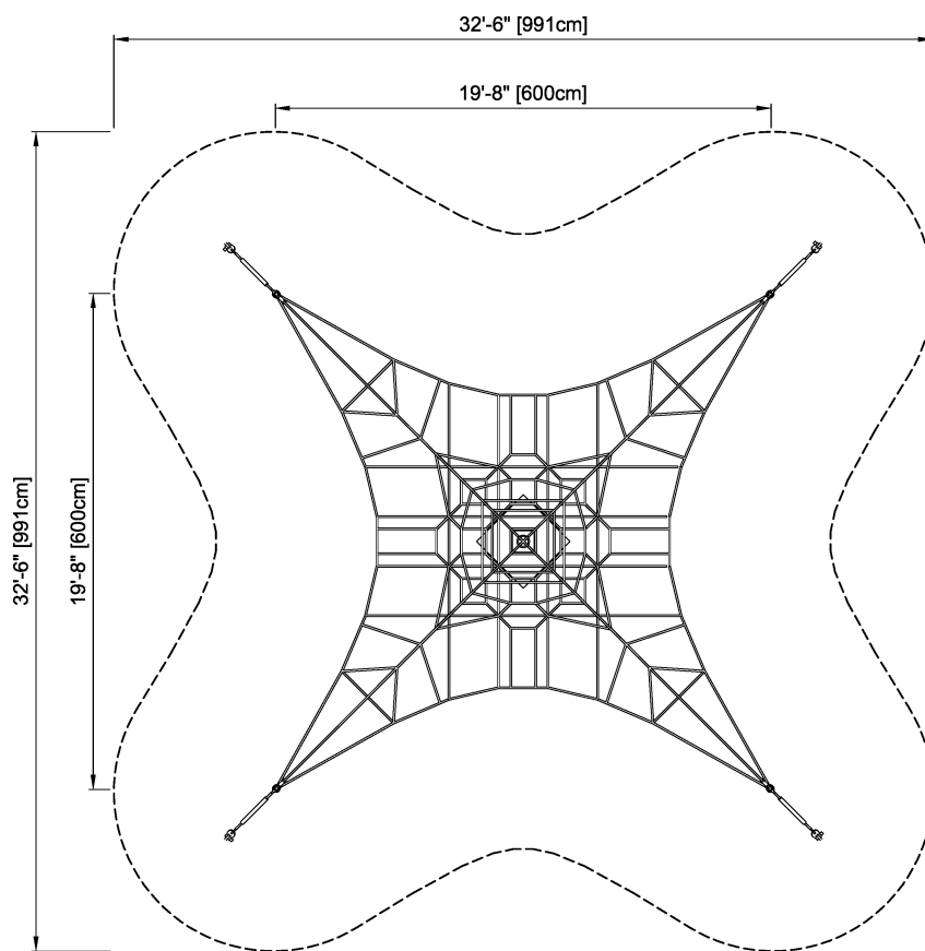
COR303011 * 3'-11" / 120cm ** 12'-8" / 385cm ***847.1ft 2 / 80.6m 2 1:100
